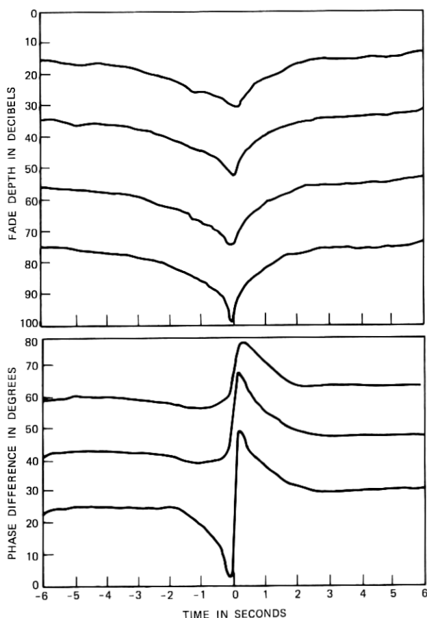
Fig. 6—Dispersive fading.
